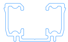
104393 Track (Champagne Only)
